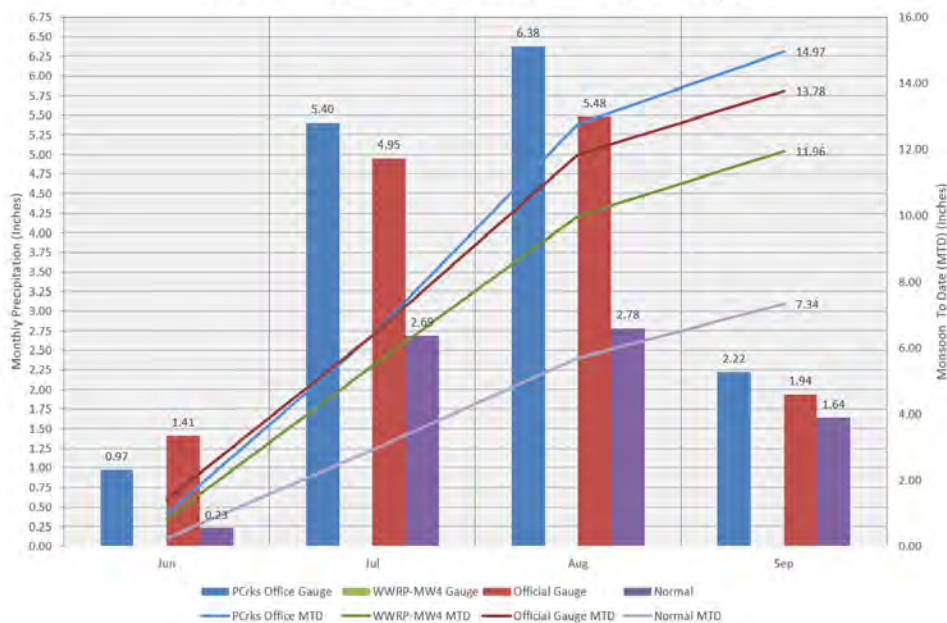
2022 - Monsoon Precipitation at Watson Woods Riparian Preserve, Prescott Creeks Office, & NOAA Official Rain Gauges
